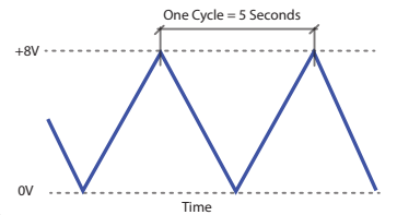
Figure 21: A Low Frequency Oscillator
